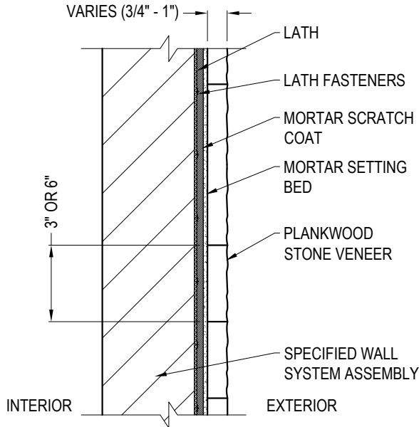
TYPICAL SECTION
