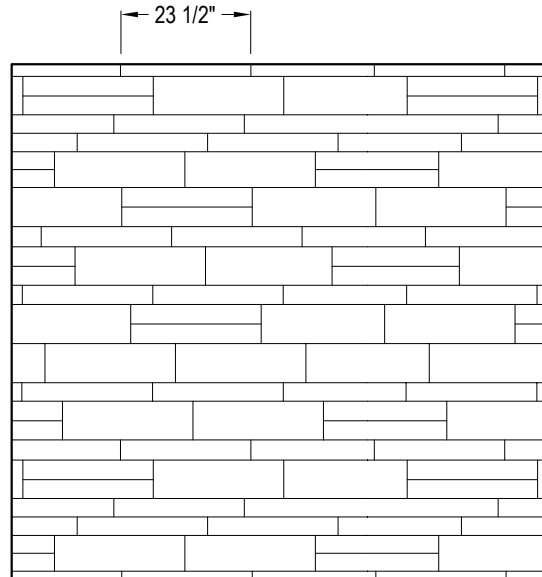
PATTERN - PLANKWOOD
