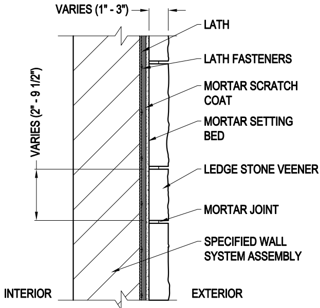
TYPICAL SECTION
