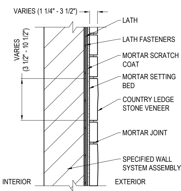
TYPICAL SECTION
