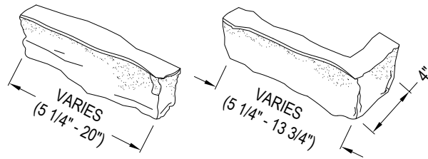
FLAT DETAIL
