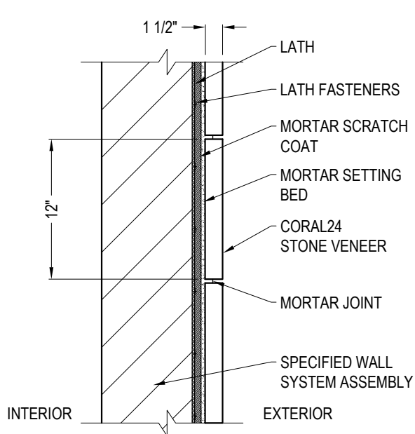
TYPICAL SECTION
